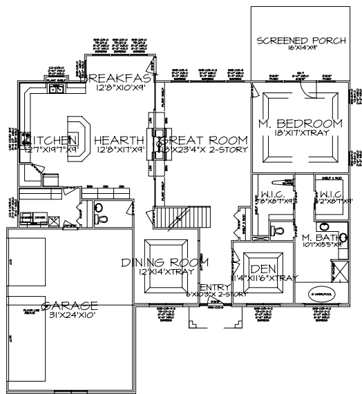
FIRST FLOOR PLAN SCALE: 1/4"=1'-0" AREA: 516 S.F. (BASEMENT) 600 S.F. (TOTAL)
