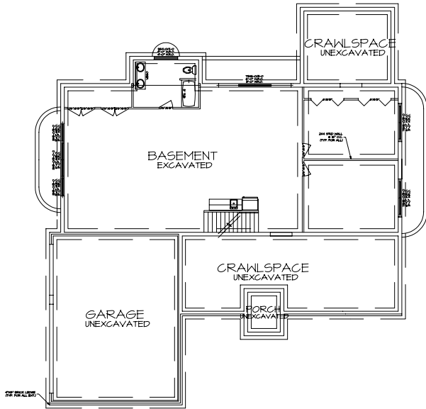
FOUNDATION PLAN SCALE: 1/4"=1'-0" AREA: 516 S.F. (BASEMENT) 600 S.F. (TOTAL) FOUNDATION PLAN NOTE: 1. ALL FOUNDATION WALLS SHALL BE CONCRETE WITH REINFORCING BARS. 2. ALL FOUNDATION WALLS SHALL BE FINISHED WITH INTERIOR BRICK OR STONE. 3. ALL FOUNDATION WALLS SHALL BE FINISHED WITH EXTERIOR BRICK OR STONE. 4. ALL FOUNDATION WALLS SHALL BE FINISHED WITH INTERIOR PLASTER AND PAINT. 5. ALL FOUNDATION WALLS SHALL BE FINISHED WITH EXTERIOR PLASTER AND PAINT. 6. ALL FOUNDATION WALLS SHALL BE FINISHED WITH INTERIOR BRICK OR STONE. 7. ALL FOUNDATION WALLS SHALL BE FINISHED WITH EXTERIOR BRICK OR STONE. 8. ALL FOUNDATION WALLS SHALL BE FINISHED WITH INTERIOR PLASTER AND PAINT. 9. ALL FOUNDATION WALLS SHALL BE FINISHED WITH EXTERIOR PLASTER AND PAINT. 10. ALL FOUNDATION WALLS SHALL BE FINISHED WITH INTERIOR BRICK OR STONE. 11. ALL FOUNDATION WALLS SHALL BE FINISHED WITH EXTERIOR BRICK OR STONE. 12. ALL FOUNDATION WALLS SHALL BE FINISHED WITH INTERIOR PLASTER AND PAINT. 13. ALL FOUNDATION WALLS SHALL BE FINISHED WITH EXTERIOR PLASTER AND PAINT. 14. ALL FOUNDATION WALLS SHALL BE FINISHED WITH INTERIOR BRICK OR STONE. 15. ALL FOUNDATION WALLS SHALL BE FINISHED WITH EXTERIOR BRICK OR STONE.
